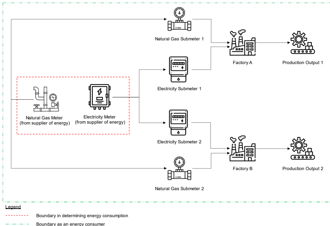
Figure 10: One or more energy or energy resources measured at one or more measuring point, supplied through a submetering to a different person who is not a related corporation but located within the same compound, to produce a production output.
